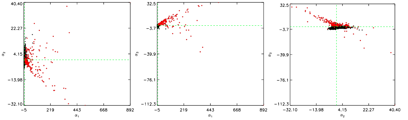
Figure 25. The admixture coefficients corresponding to PC1 ( \alpha_1 ), PC2 ( \alpha_2 ), and PC3 ( \alpha_3 ) for the Kr dataset (Sec. 3.2). Variable stars are marked in red.
