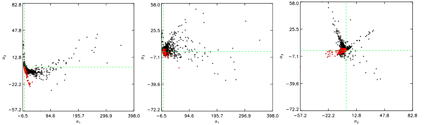
Figure 23. The admixture coefficients corresponding to PC1 ( \alpha_1 ), PC2 ( \alpha_2 ), and PC3 ( \alpha_3 ) for the TF1 dataset (Sec. 3.1). Variable stars are marked in red.
