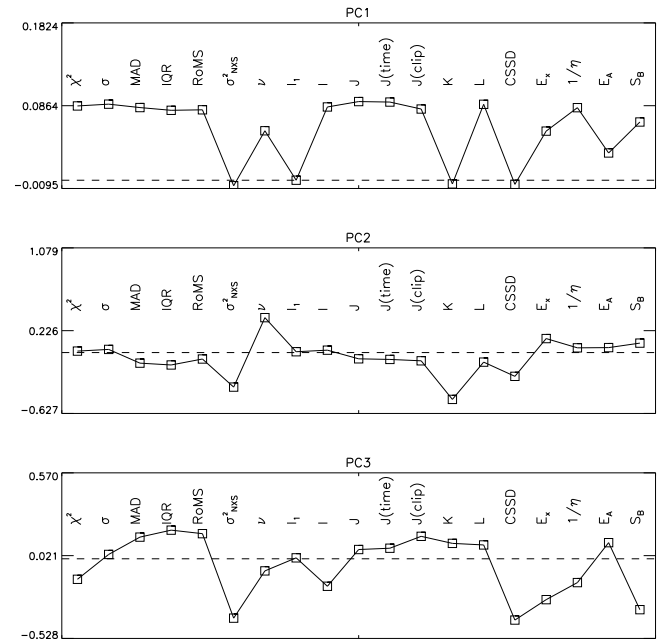
Figure 7. The first three principal components in the Kr dataset (Sec. 3.2). The dashed line indicates zero contribution of an index to the PC. Similar plots for the other datasets may be found at http://scan.sai.msu.ru/~kirx/var_idx_paper/
