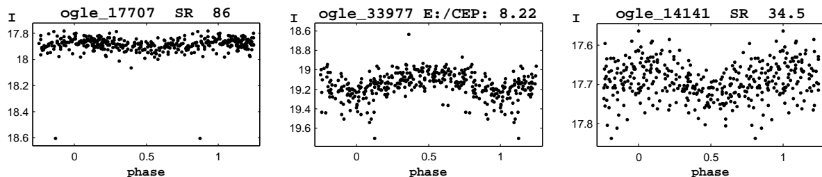
Figure 2. Lightcurves of new variable stars found in the test datasets (the complete figure is available online). The magnitudes measured in a band indicated in the top-left corner of each panel are plotted as a function of time (Julian day) for irregular or phase for periodic variables. The title of each panel indicate the object identifier in Table 4, its variability type and period in days (if applicable).
