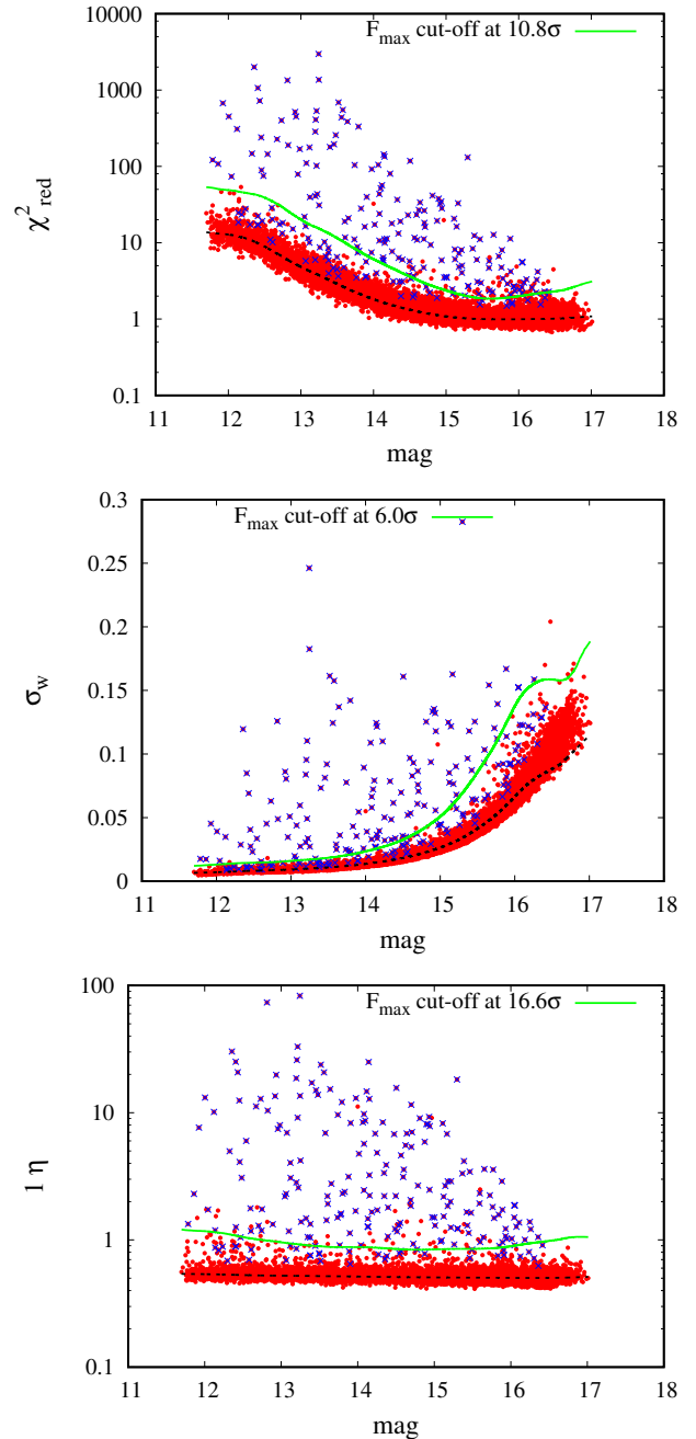
Figure 3. Variability indices \chi_{\text{red}}^2 (Sec. 2.1), \sigma_w (Sec. 2.2), and 1/\eta (Sec. 2.15) plotted as a function of magnitude for the Krasnoyarsk dataset (Sec. 3.2). Variable stars are marked with ‘x’. The curves represent the expected value of \chi_{\text{red}}^2 , \sigma_w , and 1/\eta for a given magnitude and the selection threshold corresponding to the best trade-off between the completeness and purity of the candidates list ( F_{\max} ; see Sec. 4, Fig. 4). The index–magnitude plots for the other indices and datasets may be found online at http://scan.sai.msu.ru/~kirx/var_idx_paper/
