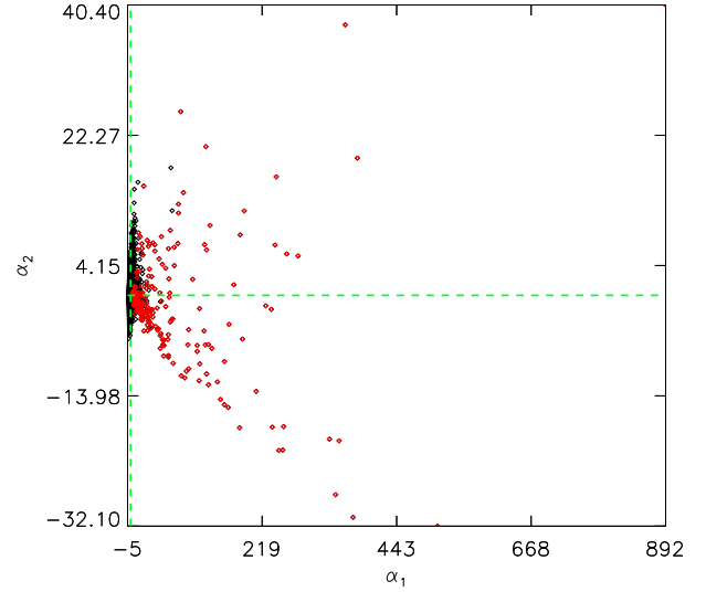
Figure 6. The admixture coefficients corresponding to PC1 ( \alpha_1 ), PC2 ( \alpha_2 ) for the Kr dataset (Sec. 3.2). Variable stars are marked in red. Similar plots for PC3 ( \alpha_3 ) and the other datasets may be found at http://scan.sai.msu.ru/~kirx/var_idx_paper/
