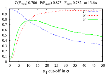
Figure 8. Variable star selection completeness (C), purity (P), and F_1 -score (F; see Sec. 4) as a function of selection threshold for the admixture coefficient \alpha_1 used as a composite variability index (Sec. 5.4) computed for the Kr dataset (Sec. 3.2). Similar plots for the other datasets may be found online at http://scan.sai.msu.ru/~kirx/var_idx_paper/
