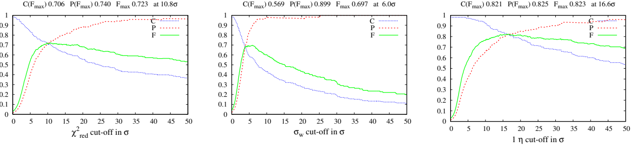
Figure 4. Variable star selection completeness (C), purity (P), and F_1 -score (F; see Sec. 4) as a function of selection threshold for the variability indices \chi^2_{\text{red}} (Sec. 2.1), \sigma_w (Sec. 2.2), and 1/\eta (Sec. 2.15) computed for the Krasnoyarsk dataset (Sec. 3.2). C-, P-, and F_1 -score plots for the other indices and datasets may be found online at http://scan.sai.msu.ru/~kirx/var_idx_paper/
