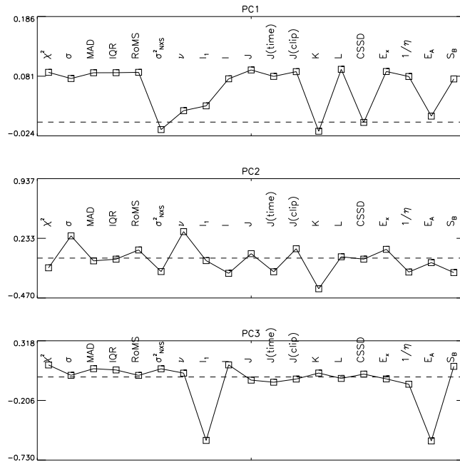
Figure 33. The first three principal components in the the OGLE dataset (Sec. 3.5). The dashed line indicates zero contribution of an index to the PC. Percentage of the total variance explained by PC1/PC2/PC3: 55.1/10.8/7.7.
