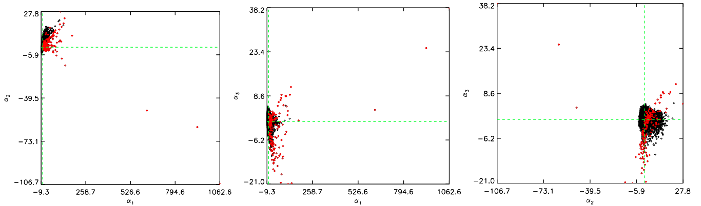
Figure 27. The admixture coefficients corresponding to PC1 ( \alpha_1 ), PC2 ( \alpha_2 ), and PC3 ( \alpha_3 ) for the OGLE dataset (Sec. 3.5). Variable stars are marked in red.
