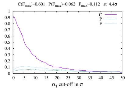
Figure 35. Variable star selection completeness (C), purity (P), and F_1 -score (F; see Sec. 4) as a function of selection threshold for the admixture coefficient \alpha_1 used as a composite variability index (Sec. 5.4) computed for the TF1 dataset (Sec. 3.1).
