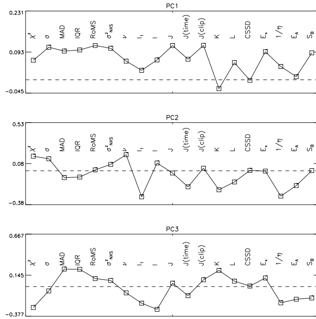
Figure 34. The first three principal components in the the 66Oph dataset (Sec. 3.6). The dashed line indicates zero contribution of an index to the PC. Percentage of the total variance explained by PC1/PC2/PC3: 42.3/13.9/10.6.
