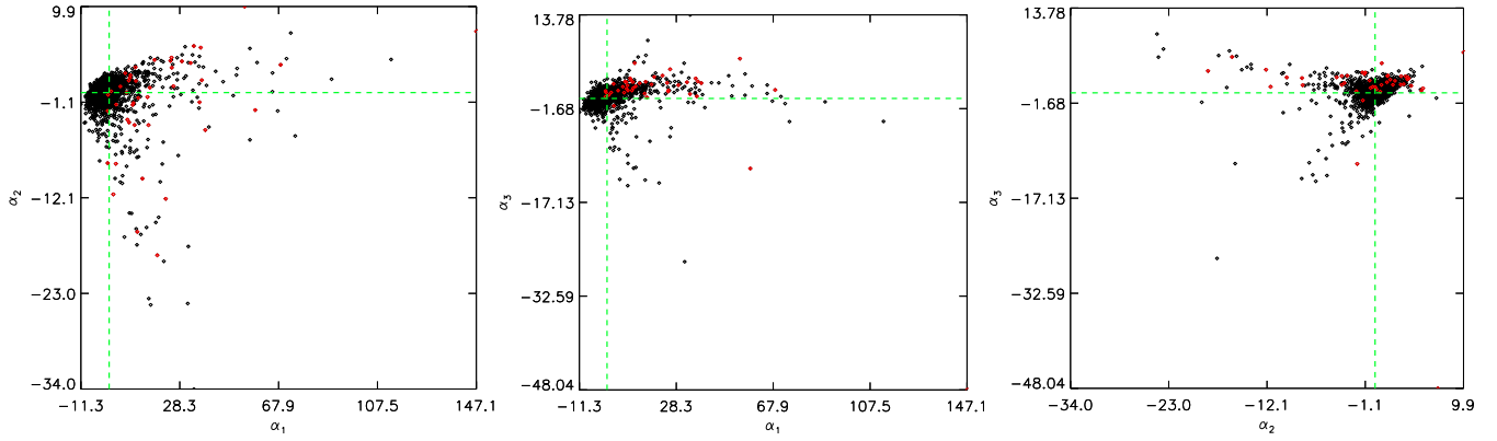
Figure 25. The admixture coefficients corresponding to PC1 ( \alpha_1 ), PC2 ( \alpha_2 ), and PC3 ( \alpha_3 ) for the W1 dataset (Sec. 3.3). Variable stars are marked in red.
