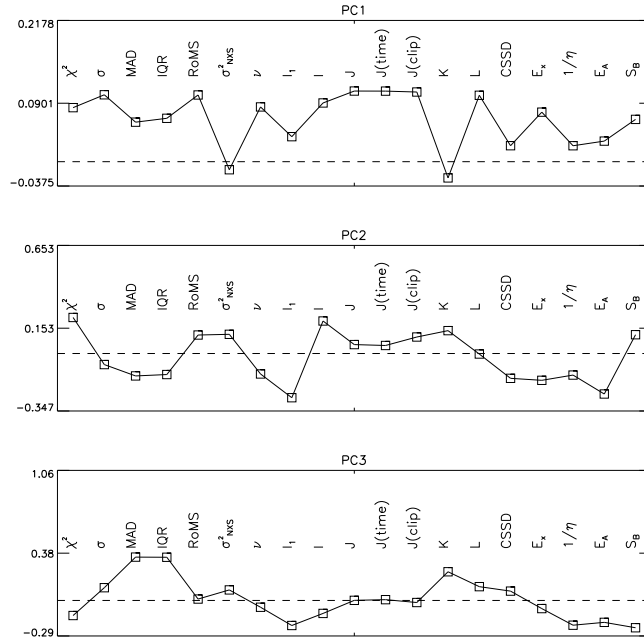
Figure 30. The first three principal components in the the TF2 dataset (Sec. 3.1). The dashed line indicates zero contribution of an index to the PC. Percentage of the total variance explained by PC1/PC2/PC3: 47.0/12.9/9.9.
