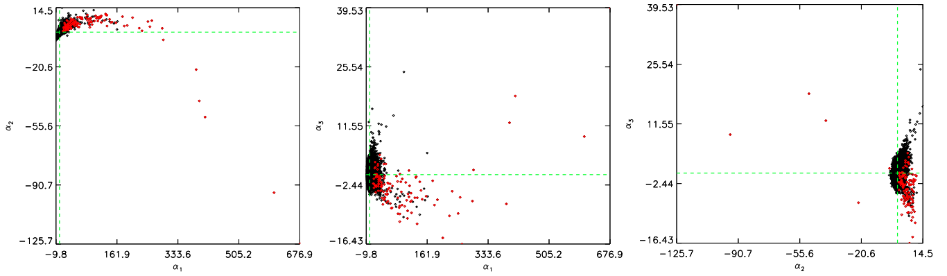
Figure 26. The admixture coefficients corresponding to PC1 ( \alpha_1 ), PC2 ( \alpha_2 ), and PC3 ( \alpha_3 ) for the And1 dataset (Sec. 3.4). Variable stars are marked in red.
