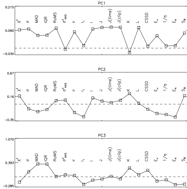
Figure 29. The first three principal components in the the TF1 dataset (Sec. 3.1). The dashed line indicates zero contribution of an index to the PC. Percentage of the total variance explained by PC1/PC2/PC3: 47.8/11.0/9.3.
