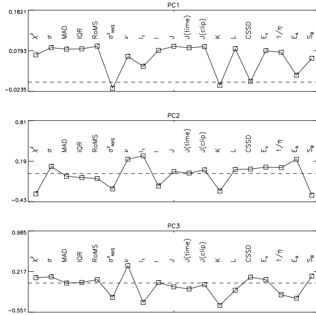
Figure 32. The first three principal components in the the And1 dataset (Sec. 3.4). The dashed line indicates zero contribution of an index to the PC. Percentage of the total variance explained by PC1/PC2/PC3: 55.9/8.8/7.2.
