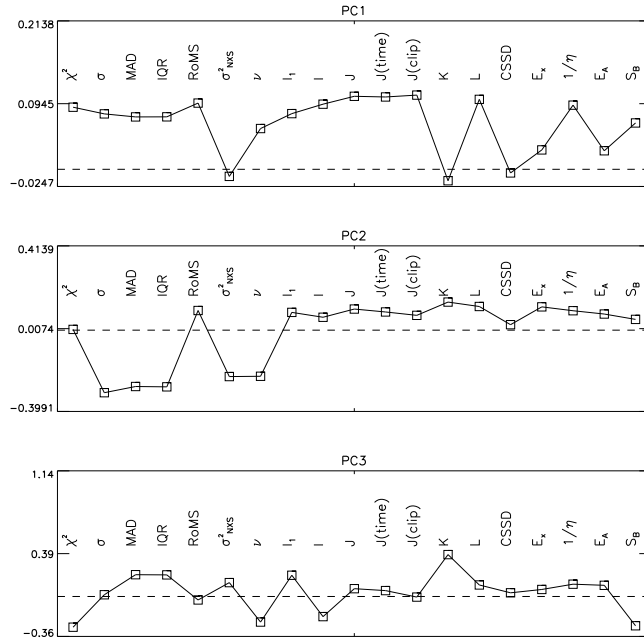
Figure 31. The first three principal components in the the W1 dataset (Sec. 3.3). The dashed line indicates zero contribution of an index to the PC. Percentage of the total variance explained by PC1/PC2/PC3: 47.0/11.4/9.4.
