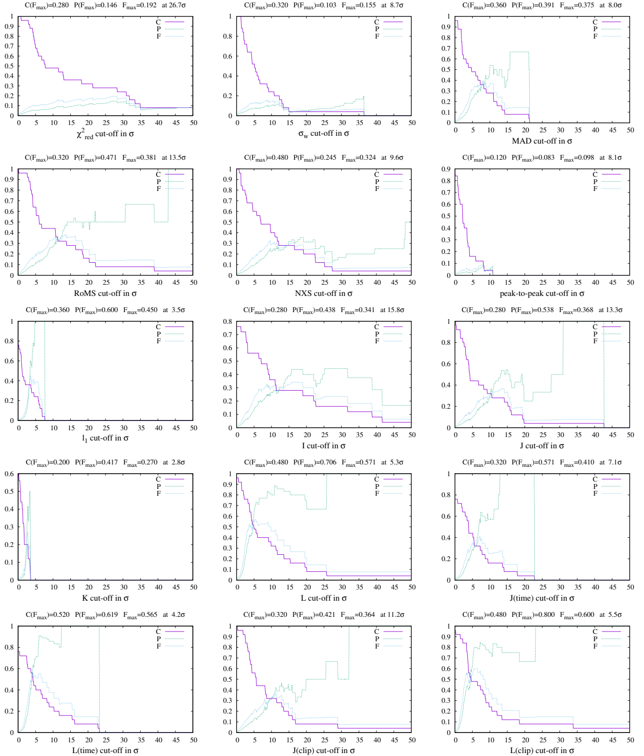
Figure 22. Variable star selection completeness (C), purity (P), and F_1 -score (F, see Sec 4) as a function of selection threshold for the variability indices defined in Sec. 2 (66 Oph dataset, Sec. 3.6).
