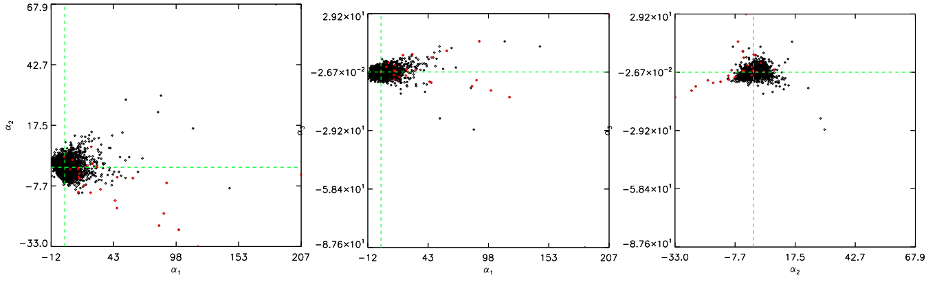
Figure 28. The admixture coefficients corresponding to PC1 ( \alpha_1 ), PC2 ( \alpha_2 ), and PC3 ( \alpha_3 ) for the 66Oph dataset (Sec. 3.6). Variable stars are marked in red.
